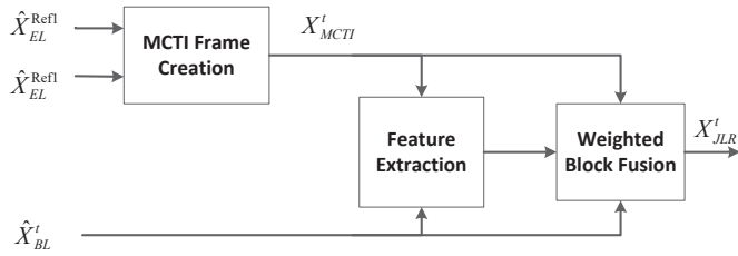
Fig. 2. Joint layer reference frame creation architecture.
