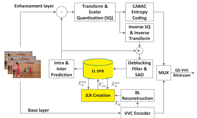
Fig. 1. Proposed QS-VVC encoder architecture.
